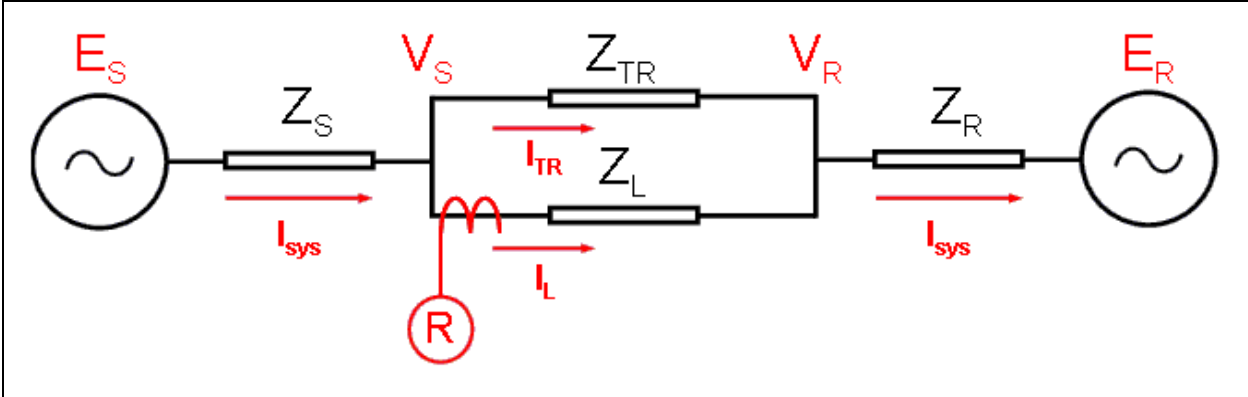
Figure 3. System impedance as seen by relay R.
