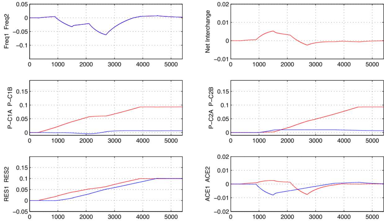
Figure 31. Response to load ramps - Limited primary response headroom - LFC active 20 percent of capacity in each BA provides primary response and pre-scheduled ramping of output 20 percent of capacity in each BA provides primary response but no secondary response
