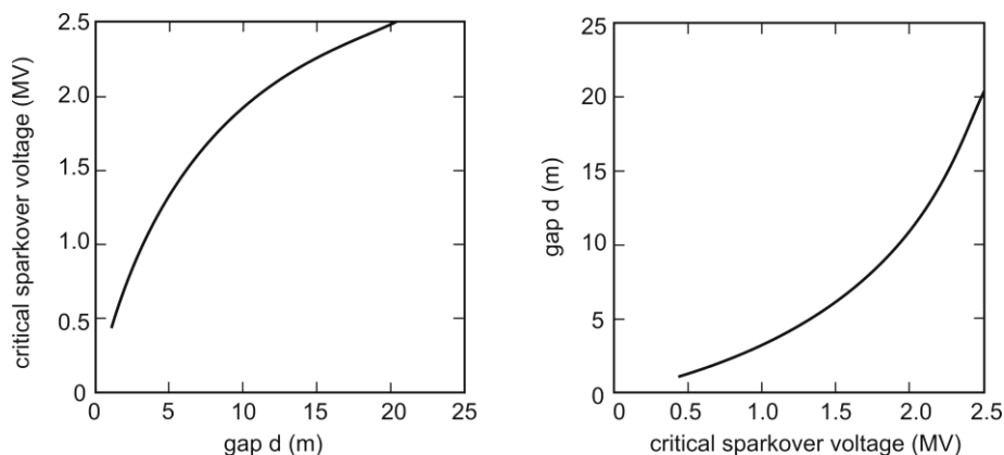
(a) The Gallet equation solved
