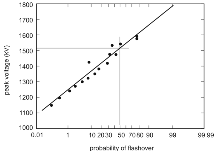
Figure 2 Representative flashover probability data.
