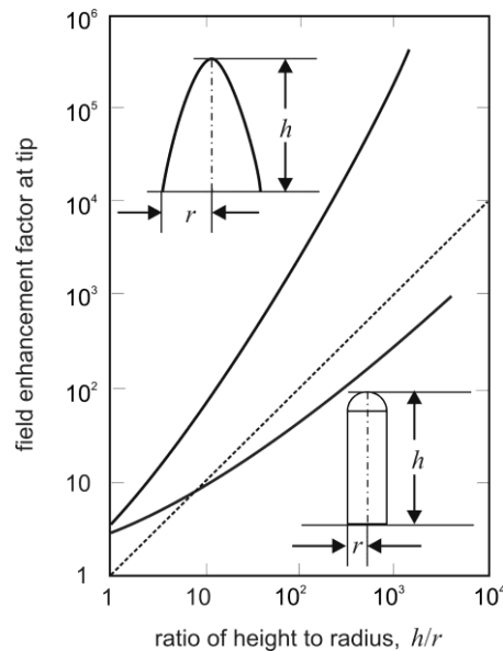
Figure 17 Field enhancement factors
