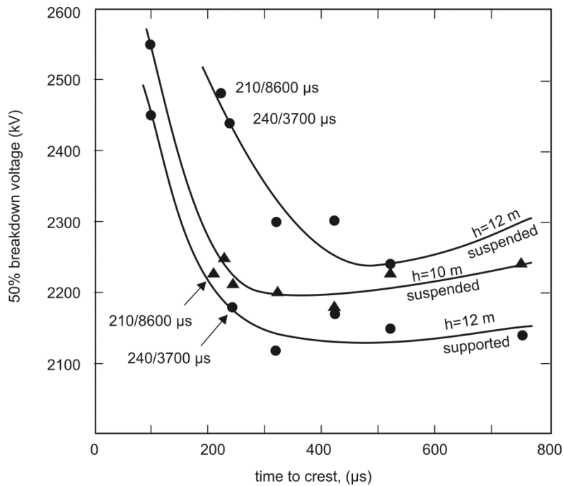
Figure 10 Variation of voltage withstand with pulse shape
