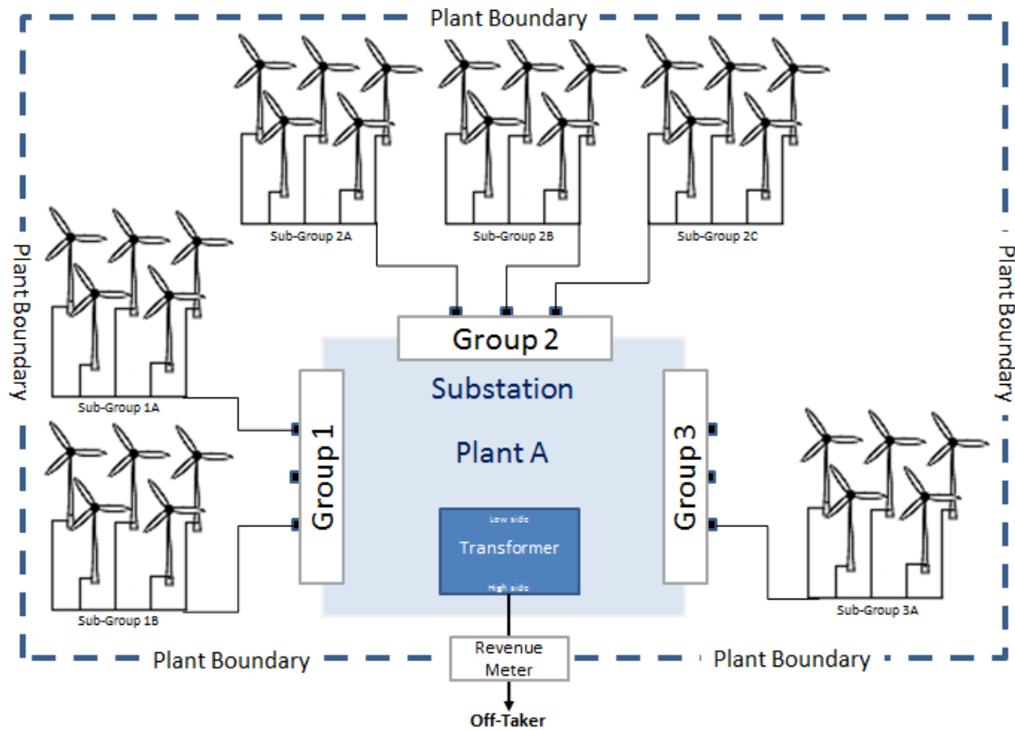
Figure 2: Typical Wind Plant Layout
