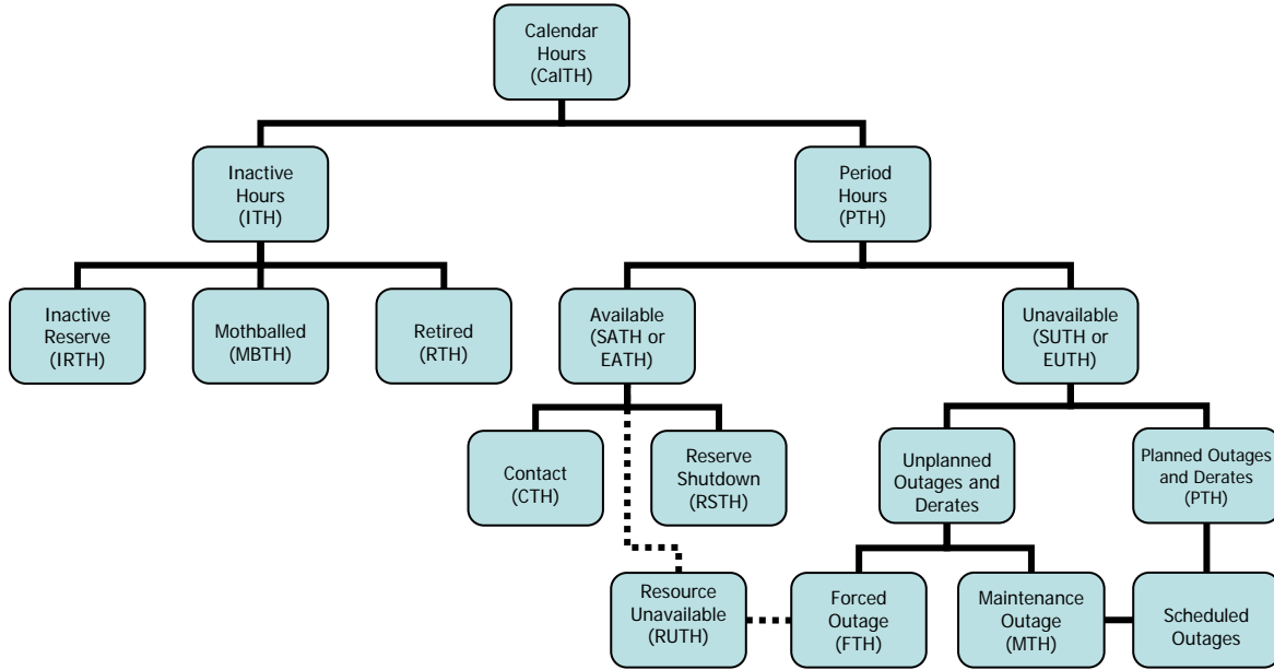
Figure D-1 Time Spent in Various Turbine Unit States
